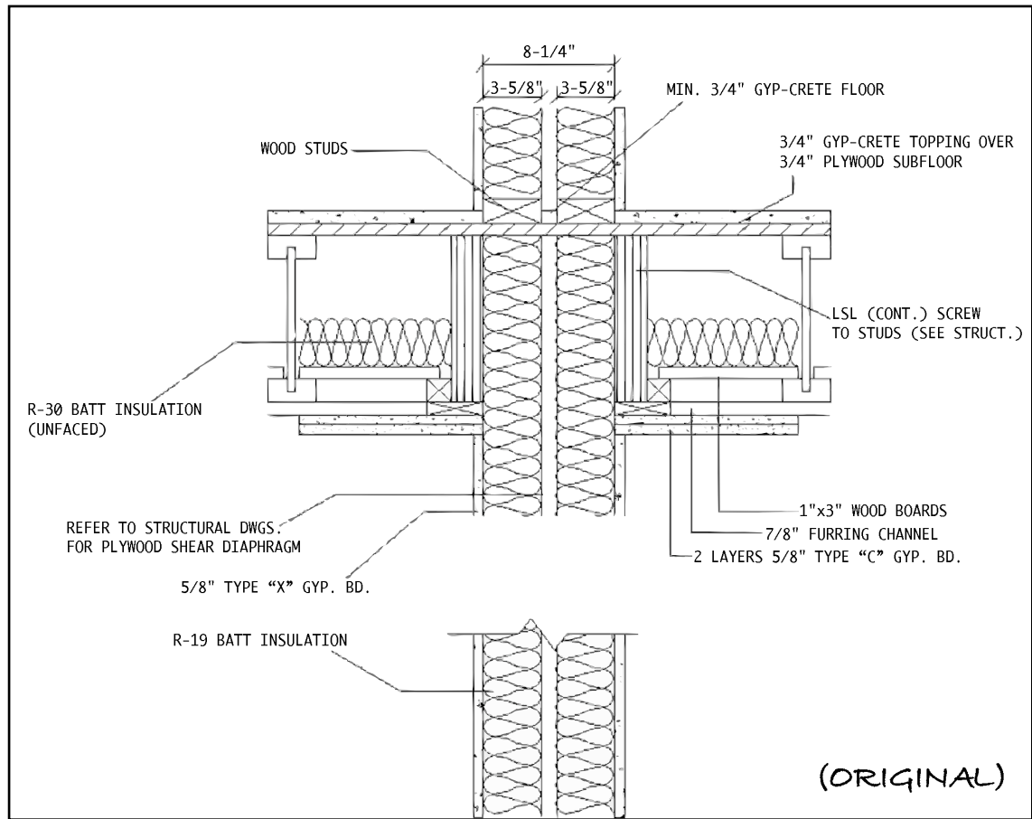
WALL CONSTRUCTION DETAILS JEFF DRAKE, 15 OCT 2001
